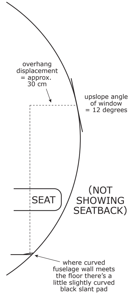
VIEW ALONG FUSELAGE LOOKING FORWARD
